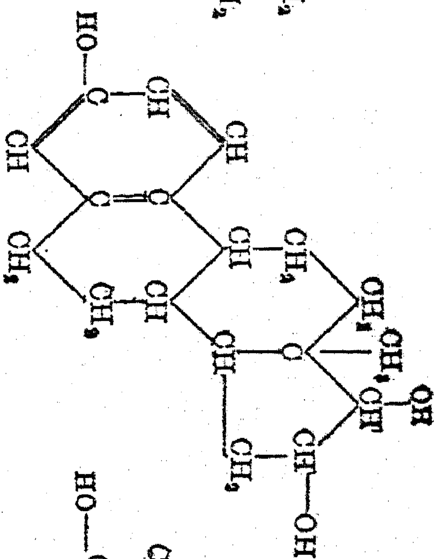
II. Follikelhormonhydrat
