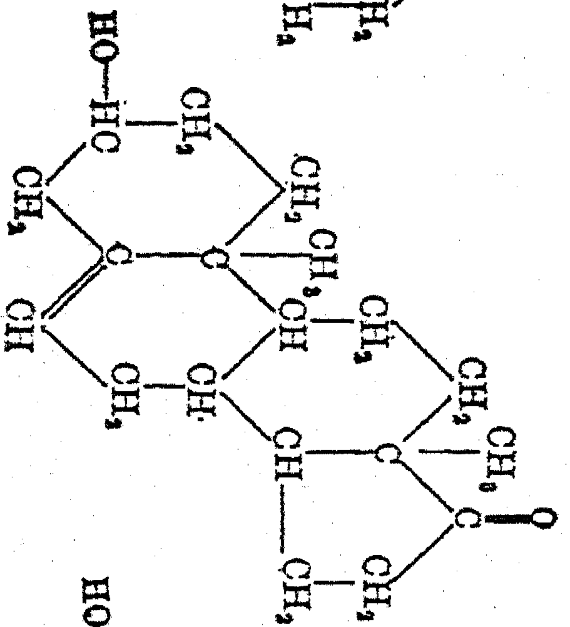
VII. Dehydroandrosteron
