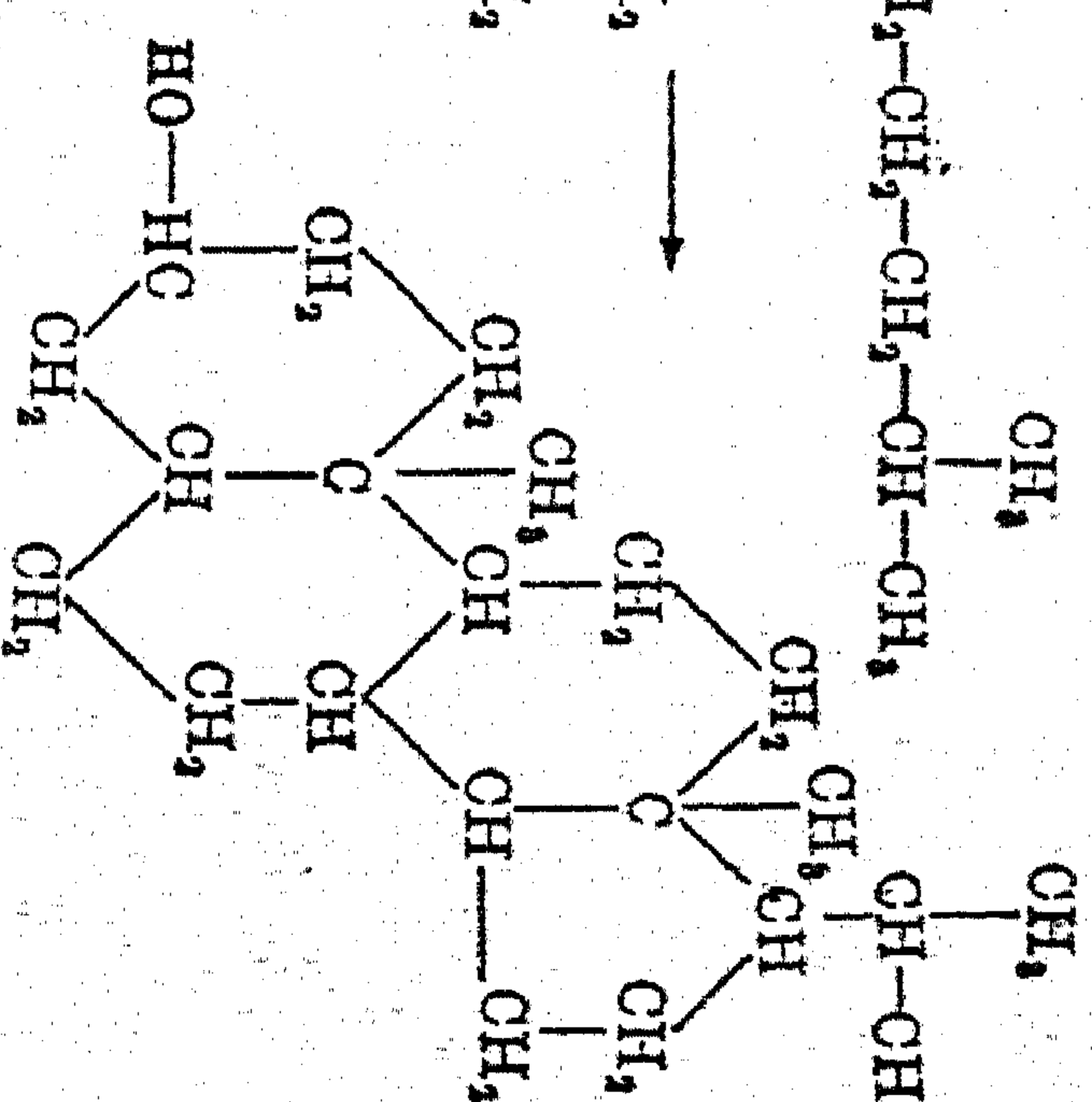
IX. epi-Dihydrocholesterin
