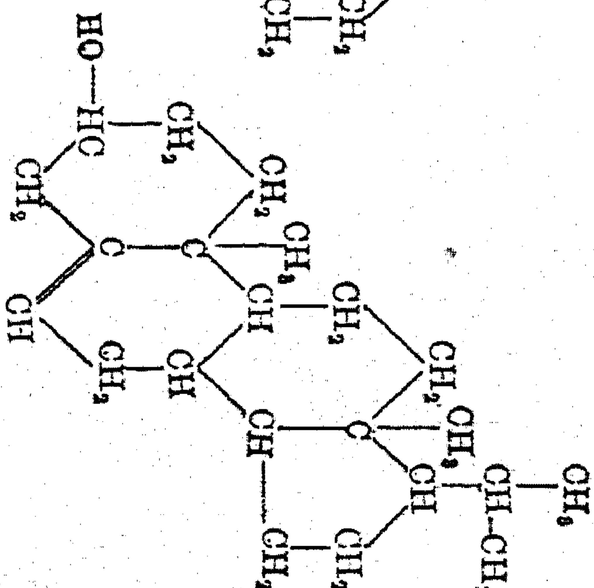
VIII. Cholosterin
