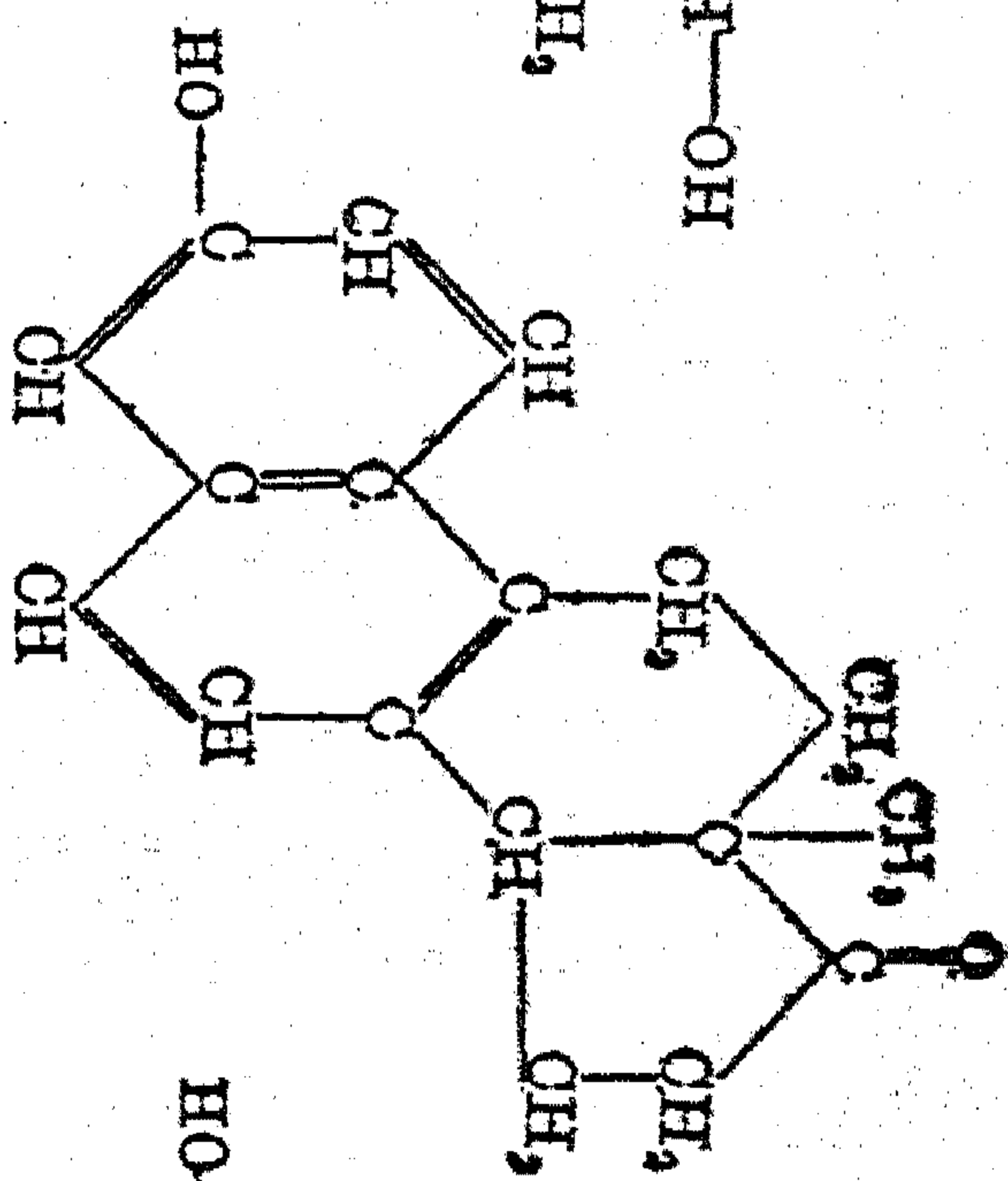
III. Equilenin
