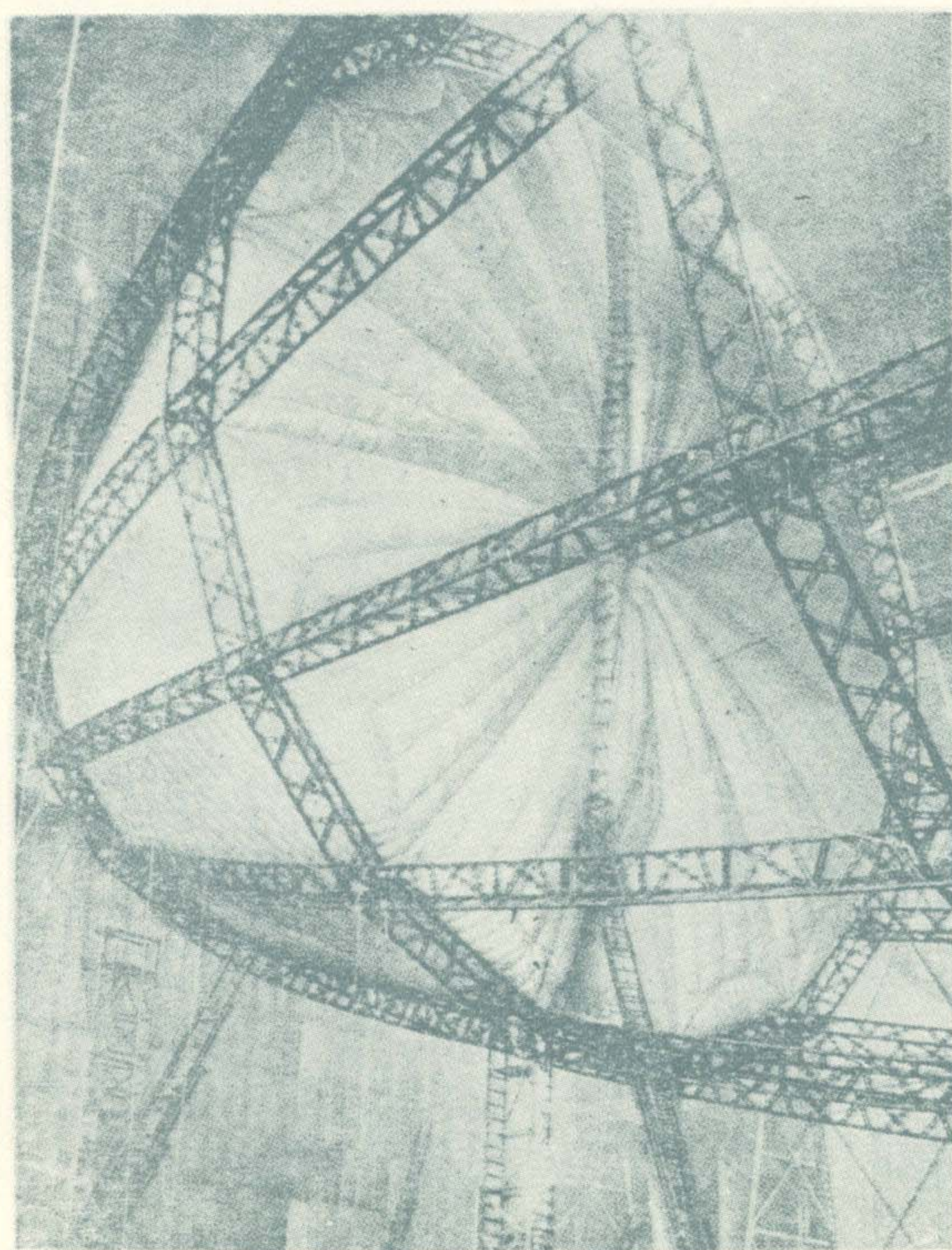
Anovel view of the R100, the largest airshib everbilt, which is now under construction in Yorkshire.
