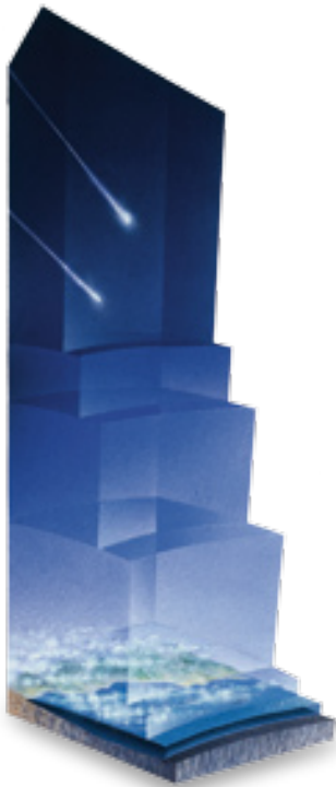
Layers of Earth's atmosphere
