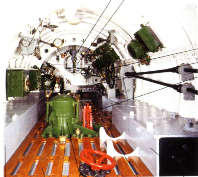
Distilled water tank Wooden deckboard Log tank Cradle for oxygen bottle Freshwater tank
