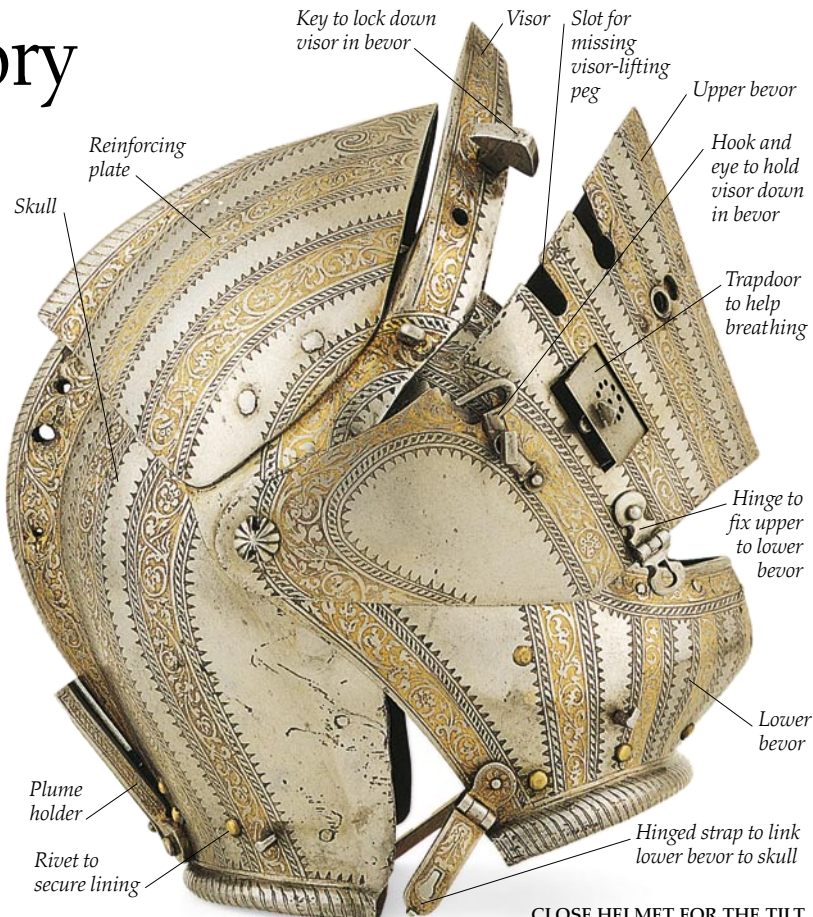
CLOSE HELMET FOR THE TILT This etched North Italian helmet of about 1570 has a reinforcing plate riveted to the skull or bowl. The visor fits inside the bevor, which is divided into upper and lower parts. The visor and the two parts of the bevor all pivot at the same point on each side of the skull and can be locked together.
