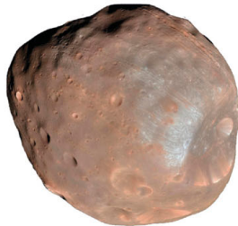
Phobos
