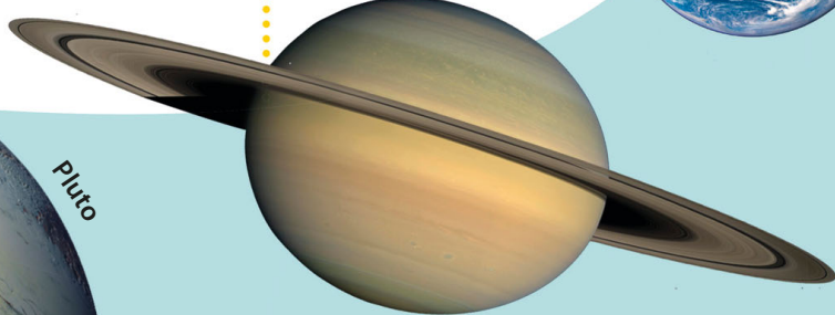
Saturn
