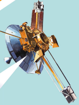
Pioneer 10
